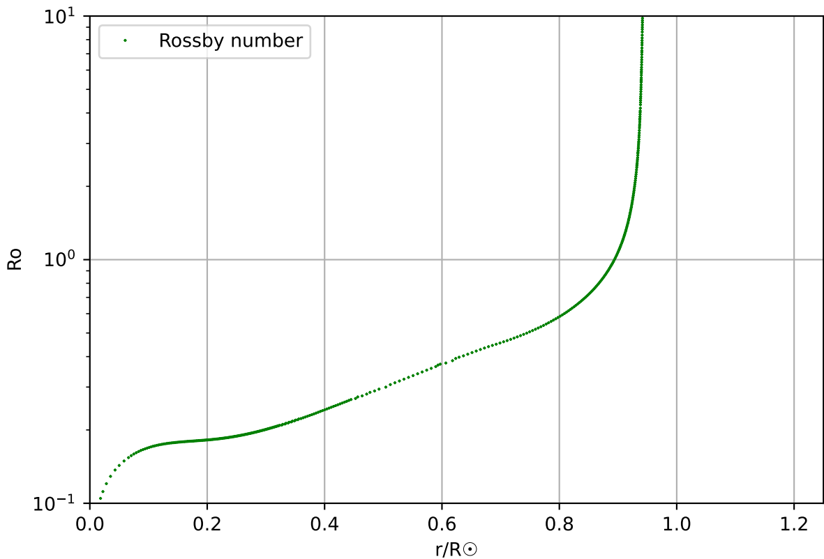
Rossby number, profile 139, age 2.69 \times 10^9
